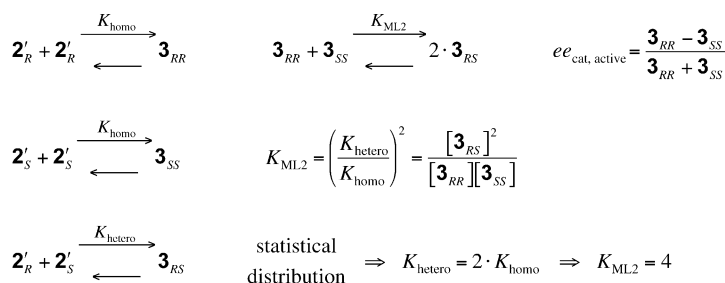
Scheme 2. Formation of dimer species 3 from the monomeric alkoxides 2' . The relationship between the equilibrium constant in Kagan's \text{ML}_2 model ( K_{\text{ML}_2} ) and the equilibrium constants for homochiral ( K_{\text{homo}} ) and heterochiral ( K_{\text{hetero}} ) dimer formation is shown. The dimers are formed with a statistical distribution and only the homochiral dimers are active as catalysts.
